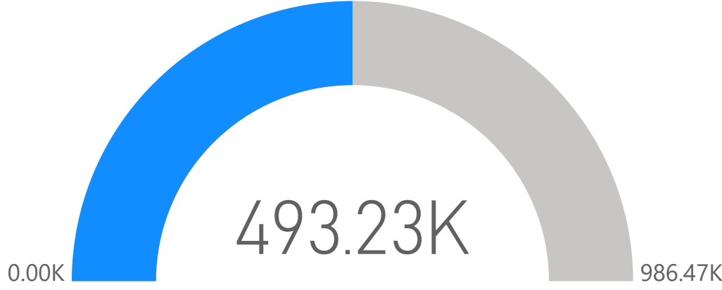
Risk_Score
